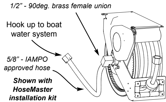
TOPMOUNT CONFIGURATION
